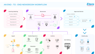
Complete workflow
